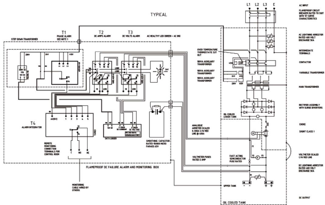
Typical ATEX (Hazardous) TR Circuit Diagram
